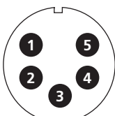
IMC2*-2005X 5 size 20
