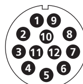
IMC2*-2212X 12 size 22
