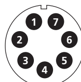
IMC2*-2007X 7 size 20
